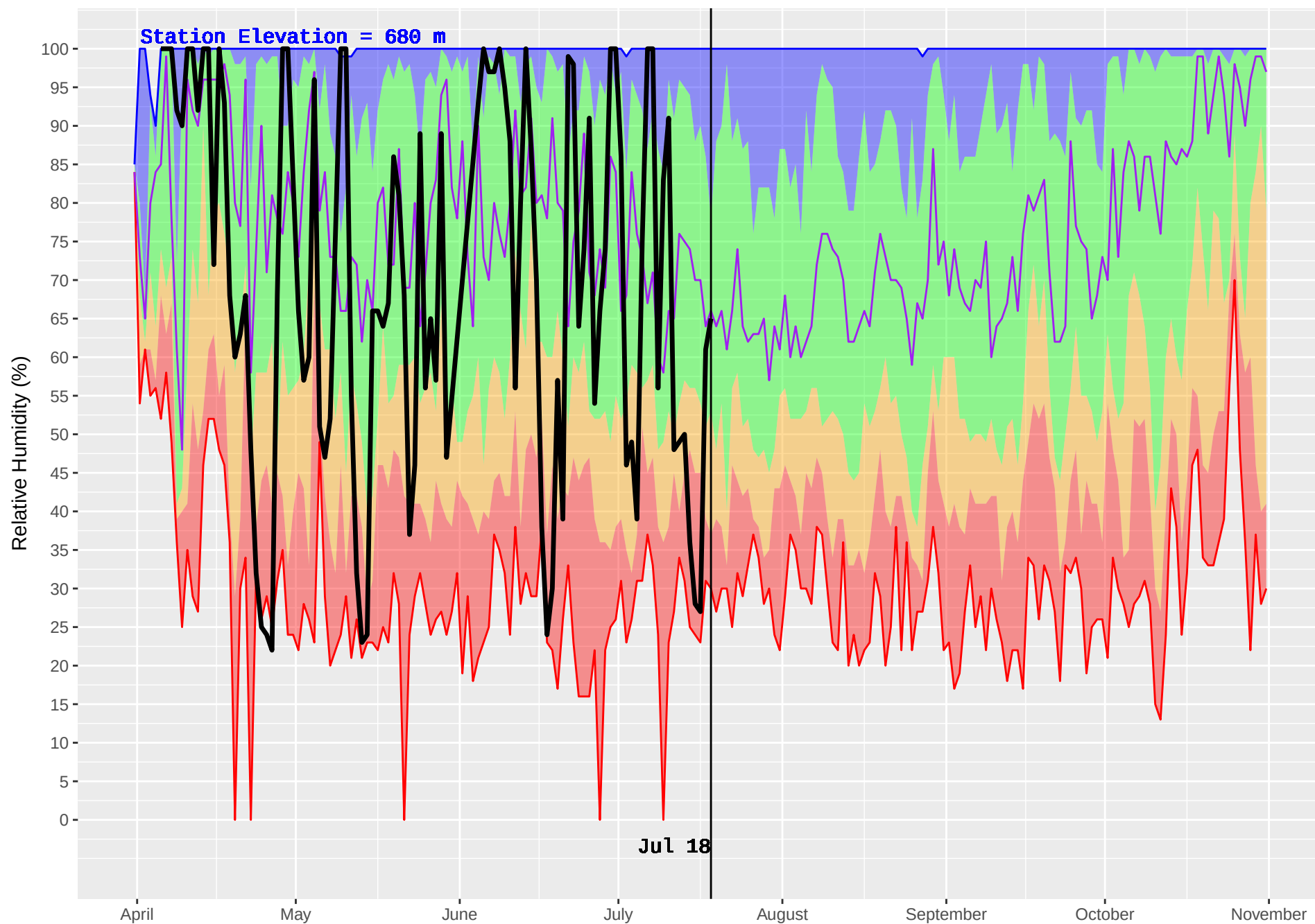
SUMMIT (11) : Historical (1985–2016) and Current (2018) Daily Relative Humidity
